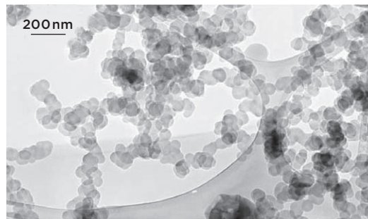
Figure 1: Microscope image of soot particles from biomass burning
