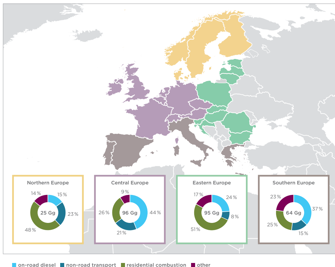
Figure 2: This figure shows the relative contributions of on-road diesel, non-road transport, and residential combustion to total black carbon emissions by region. The total annual black carbon emissions for each region is shown in gigagrams.
