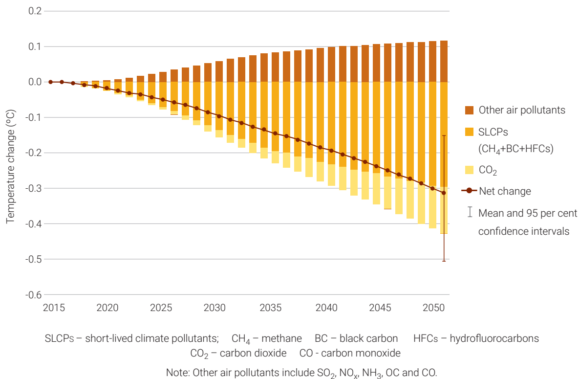
FIGURE 2.24: IMPACT OF THE DIFFERENT CLIMATE FORCERS ON GLOBAL MEAN TEMPERATURE RESULTING FROM IMPLEMENTATION OF THE TOP 25 CLEAN AIR MEASURES, COMPARED TO THE CURRENT LEGISLATION BASELINE, 2015–2050
