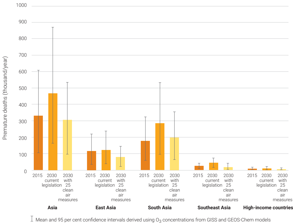
FIGURE 2.20: ESTIMATED NUMBER OF PREMATURE DEATHS ASSOCIATED WITH EXPOSURE TO O 3 IN 2015 AND IN 2030 UNDER CURRENT LEGISLATION, AND WITH THE TOP 25 CLEAN AIR MEASURES, ASIA-WIDE AND FOR THE MODELLED SUB-REGIONS
