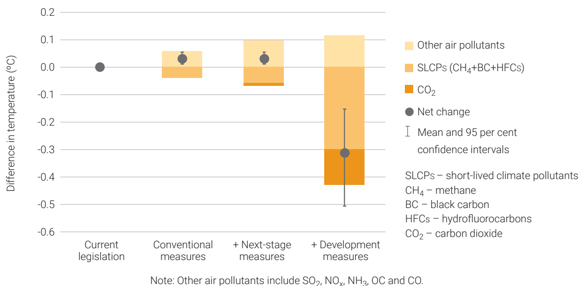
FIGURE 2.23: CHANGES IN GLOBAL MEAN TEMPERATURE IN 2050 FROM THE THREE PORTFOLIOS OF MEASURES RELATIVE TO THE CURRENT LEGISLATION BASELINE PROJECTION
