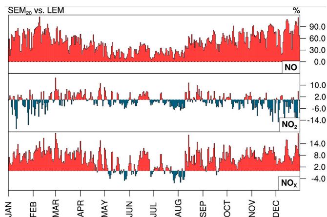
Fig. 6. Sector Explained Mass from NO x reduction level 20% ( SEM 20 ) minus the Labelled Explained Mass ( LEM ) across Germany for January to December 2018. The mass concentrations of NO (top), NO 2 (center) and NO x (bottom) have been averaged over all German background observation sites (rural, suburban, and urban). (For interpretation of the references to color in this figure legend, the reader is referred to the Web version of this article.)
