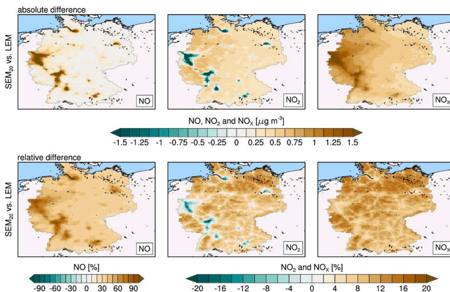
Fig. 5. Absolute (top) and relative (bottom) differences between Sector Explained Mass for NO x reduction level of 20% ( SEM 20 ) and the Labelled Explained Mass ( LEM ). From left to right: NO, NO 2 and NO x . (For interpretation of the references to color in this figure legend, the reader is referred to the Web version of this article.)
