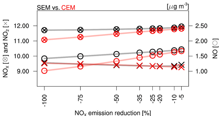
Fig. 12. Additive behavior of the source attribution for the brute force technique, of NO x reduction levels from 5 to 100%, across Germany for January to December 2018. Potential Impacts of combined emission reduction simulations (CEM) are shown in red, with potential impacts of added and individually reduced source sectors are represented in black (SEM). (For interpretation of the references to color in this figure legend, the reader is referred to the Web version of this article.)
