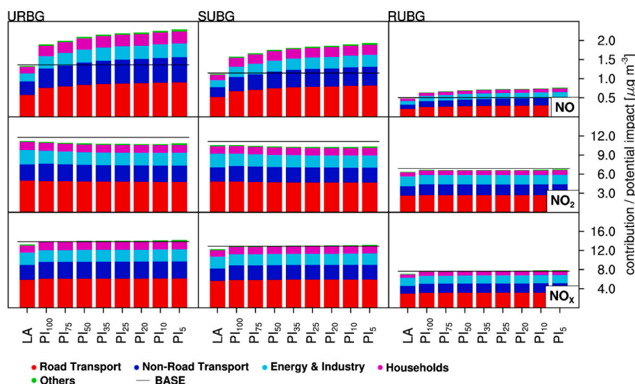
Fig. 10. Labelled contributions (LA) and potential impacts of NO x reduction levels from 5 to 100% (PI 5 , ..., PI 100 ) across Germany for January to December 2018. Three station types have been investigated and are presented from left to right (urban background: URBG, sub-urban background: SUBG, and rural background: RUBG). The mass concentration of NO (top), NO 2 (center) and NO x (bottom) have been averaged over time and space. (For interpretation of the references to color in this figure legend, the reader is referred to the Web version of this article.)
