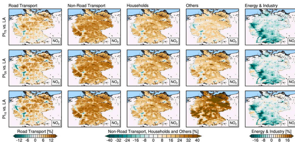
Fig. 9. Same as in Fig. 8 with relative differences and averaged in time. (For interpretation of the references to color in this figure legend, the reader is referred to the Web version of this article.)
