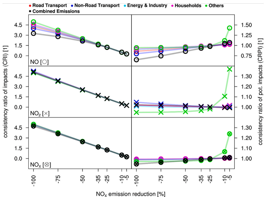
Fig. 11. Consistency ratios for impacts (left) and potential impacts (right) for NO (top), NO 2 (mid) and NO x (bottom). Sector and combined reduction simulations for 5 to 100% are divided by different colors. (For interpretation of the references to color in this figure legend, the reader is referred to the Web version of this article.)
