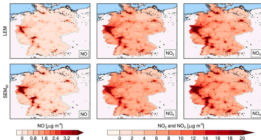
Fig. 4. Mass concentration of the Labelled Explained Mass ( LEM , top) and Sector Explained Mass for the NO x reduction level of 20% ( SEM 20 , bottom). From left to right: NO, NO 2 and NO x . (For interpretation of the references to color in this figure legend, the reader is referred to the Web version of this article.)
