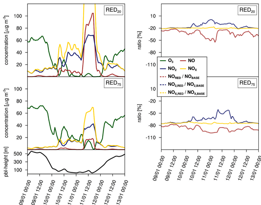
Fig. 7. Relation for NO, NO 2 , NO x and O 3 indicated for an urban background site in Berlin (capital of Germany) for 4 winter days in 2018. (For interpretation of the references to color in this figure legend, the reader is referred to the Web version of this article.)
