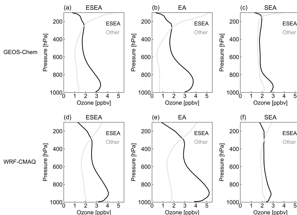
Figure 9. Vertical distribution of ozone difference contributed by anthropogenic emissions from ESEA (black) and from outside ESEA (grey) between 2019 and 1995 level, estimated from GEOS-Chem and WRF-CMAQ models. Panels (a), (b), and (c) show the results average over the ESEA domain (including East Asia domain of 80–145° E, 30–53° N and Southeast Asia domain of 92.5–135° E, 10° S–30° N), East Asia domain, and Southeast Asia domain, respectively.
