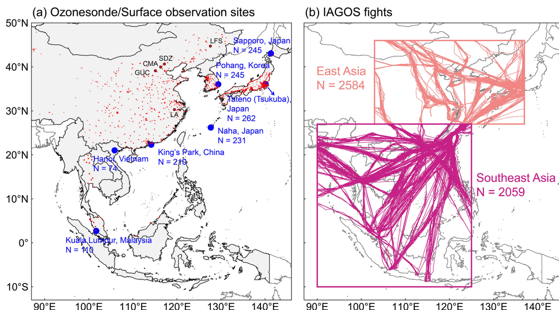
Figure 1. Tropospheric and surface ozone observations from the IAGOS, ozonesonde, and surface monitoring networks used in this study in summertime 1995–2019. Panel (a) shows the location of surface monitoring sites (red) and ozonesonde sites (blue). The small red dots represent monitoring sites from the national network; the large red dots represent the five monitoring sites in China with long-term ozone observations. Numbers of available profiles ( N ) for ozonesonde measurements are shown in the inset. Panel (b) shows the IAGOS flight tracks in the troposphere. The boxes indicate the region of East Asia (103–137° E, 27–46° N) and Southeast Asia (90–123° E, 10–27° N). Numbers of available profiles ( N ) for flight tracks are shown in the inset. Detailed information of the observations is summarized in Table 1. Areas with grey shadings in panel (a) denote ESEA countries defined in this study (Mongolia, China, Democratic People's Republic of Korea, Republic of Korea, Japan, Myanmar, Thailand, Laos, Viet Nam, the Philippines, Cambodia, Malaysia, and Indonesia).
