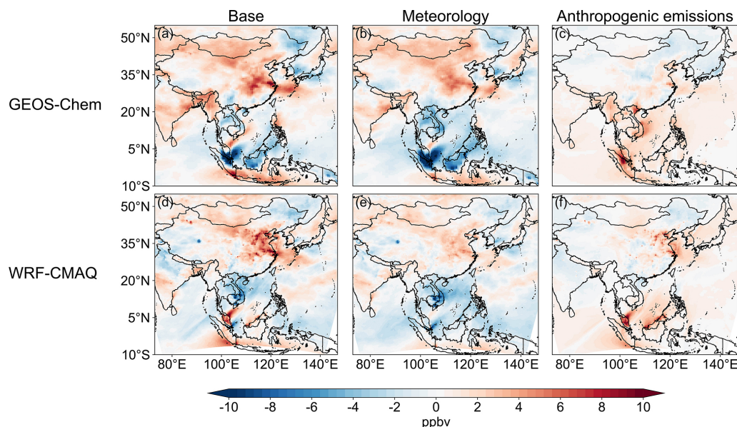
Figure 15. Differences in simulated June–August mean MDA8 ozone concentrations between 2017–2019 and 2013–2015 (2017–2019 minus 2013–2015). Panels (a), (b), and (c) show the difference-simulated surface MDA8 ozone concentration, contribution from meteorological conditions, and contribution from anthropogenic emissions, respectively, from the GEOS-Chem model. Panels (d), (e), and (f) are the same as (a), (b), and (c) but for the WRF-CMAQ model.
