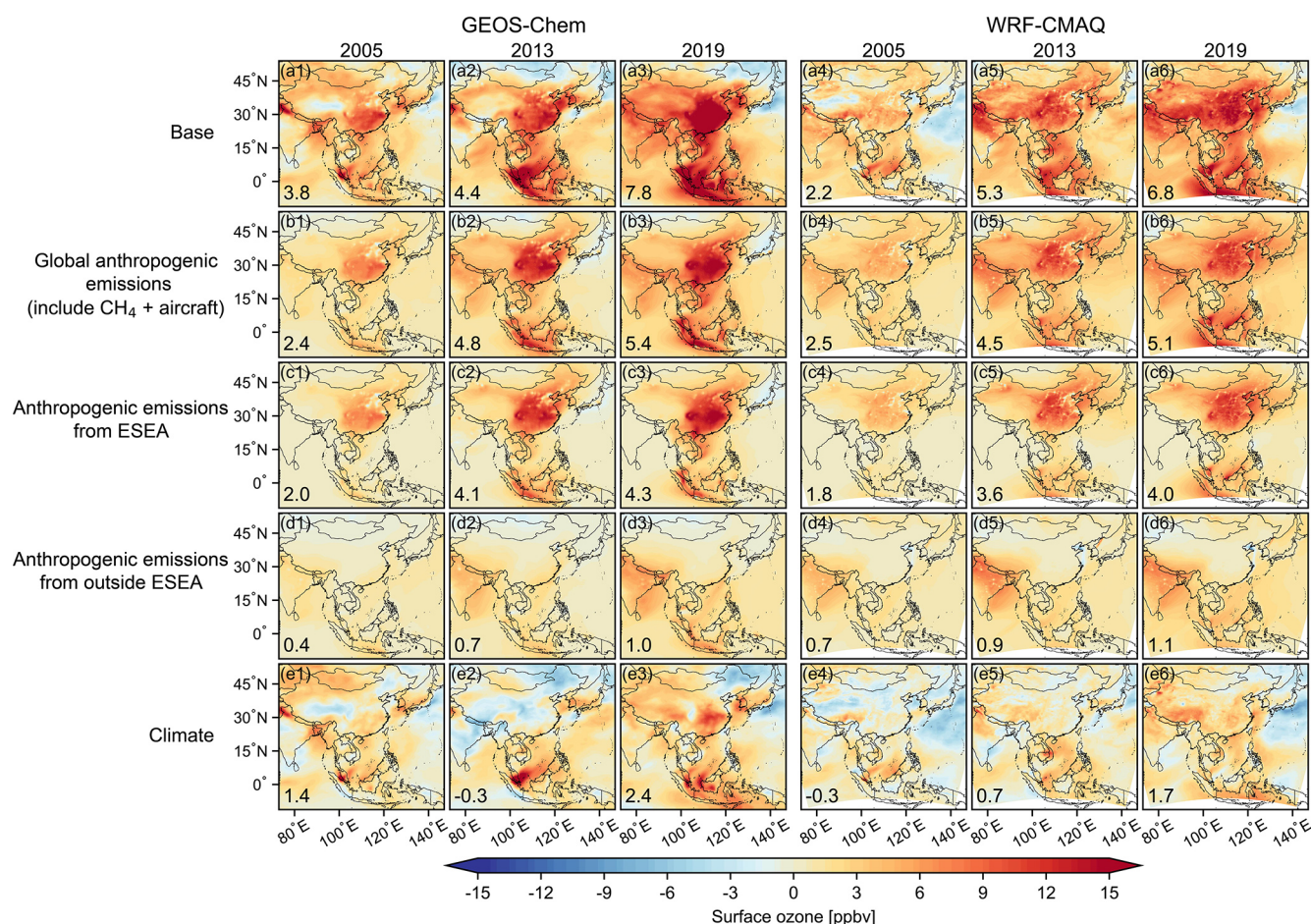
Figure 11. Same as Fig. 7 but for surface ozone.
