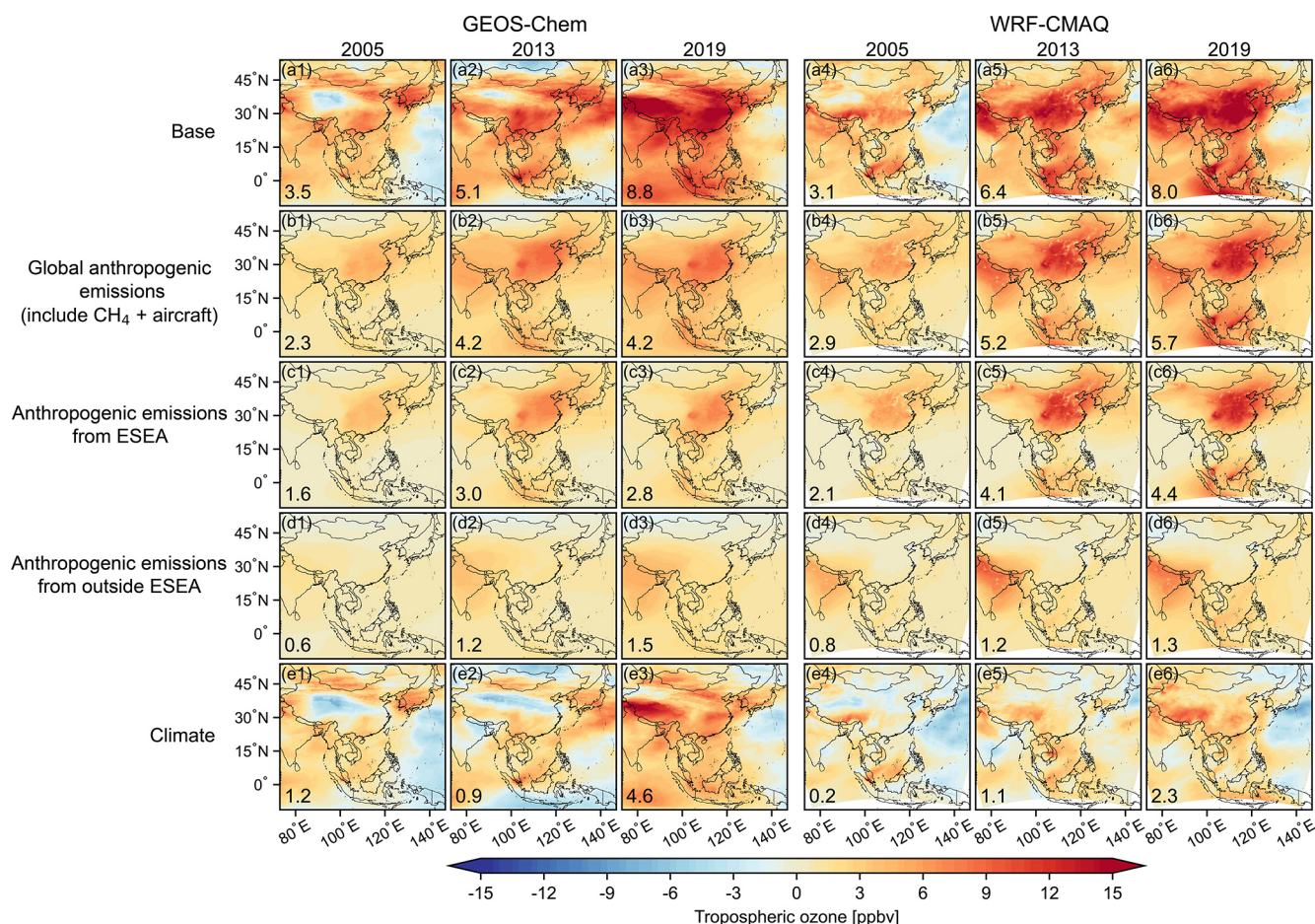
Figure 7. Factors contributing to changes in summertime tropospheric ozone column (represented as column-averaged in units of ppbv) in East Asia and Southeast Asia estimated from the GEOS-Chem and WRF-CMAQ models. Results are ozone differences between the corresponding year and 1995. Ozone differences contributed by changes in global anthropogenic emissions (including surface emissions, aircraft emissions, and methane) ( b ), anthropogenic emissions from ESEA ( c ), anthropogenic emissions from outside ESEA ( d ), and climate (including biomass burning and stratospheric influences) relative to 1995 ( e ) are estimated. Numbers are mean values across the continental ESEA.
