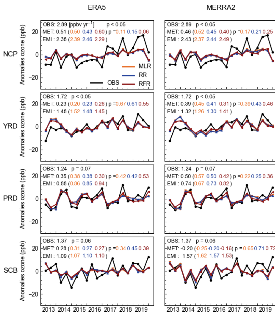
Figure 14. Trends in observed summertime ozone and model-derived meteorologically driven trends in key city clusters in China. Results are MDA8 ozone anomalies for individual JJA months averaged over the cities relative to the 2013–2019 mean. Observed trends are compared to the meteorologically driven trends diagnosed by the MLR, RR, and RFR, using ERA5 and MERRA-2 meteorological data, respectively. The observed trends and mean estimates of the trends driven by meteorology and emissions averaged over the three methods are shown in the inset, with the trends estimated by individual methods shown in parentheses. Meteorologically driven ozone trends are estimates as the linear trends of ozone concentrations predicted exclusively from meteorological variables using statistical or machine learning models. The trends of ozone residuals (subtracting the meteorologically predicted ozone from the observed ozone concentrations) are interpreted as ozone trends driven by changes in anthropogenic emissions.
