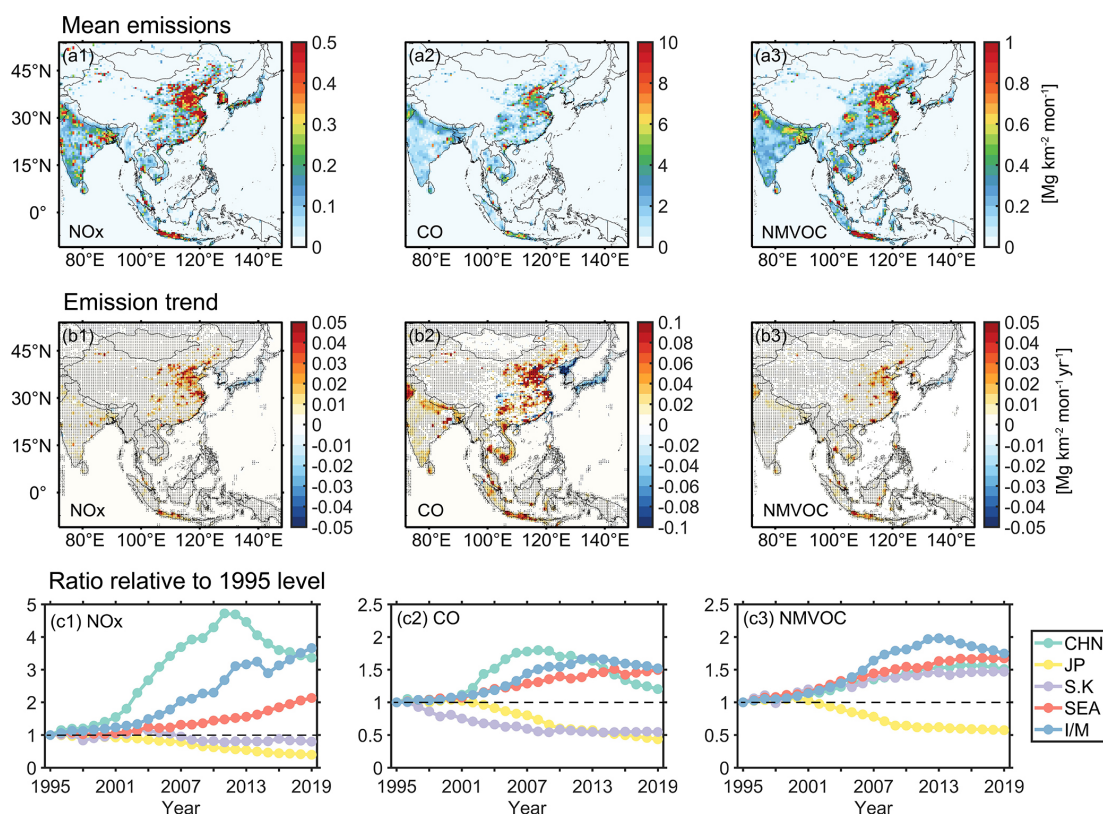
Figure 2. Spatial distributions and long-term trends in summertime anthropogenic emissions of \text{NO}_x , CO, and NMVOC in East and South-east Asia. Emission estimates are from the CEDSv2 inventory. Panels (a1)–(a3) show mean emissions averaged over years 2015, 2017, and 2019. Panels (b1)–(b3) show the 1995–2019 trends. Black dots denoted linear trends with a p value < 0.05 . Panels (c1)–(c3) show the time series of emission ratio relative to 1995 level for different regions, in which CHN stands for China, JP stands for Japan, S.K. stands for South Korea, SEA includes Myanmar, Thailand, Laos, Viet Nam, Cambodia, and Philippines, I/M stands for Indonesia and Malaysia.
