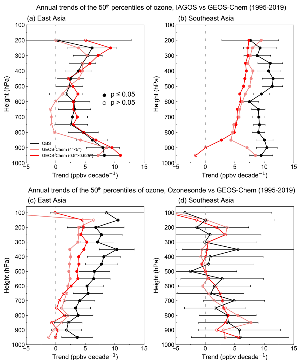
Figure 5. Evaluation of GEOS-Chem’s ability to capture summertime tropospheric ozone trends over IAGOS regions and at ozonesonde sites. Panel (a) shows trends of the 50 th percentiles of IAGOS observed and GEOS-Chem simulated summertime ozone trends (ppbv per decade) at intervals of 50 hPa in 1995–2019. The trends are calculated using the quantile regression method (Sect. 2.4). Filled circles indicate trends with p value < 0.05 . Horizontal bars represent trends at 95 % confidence level from observations.
