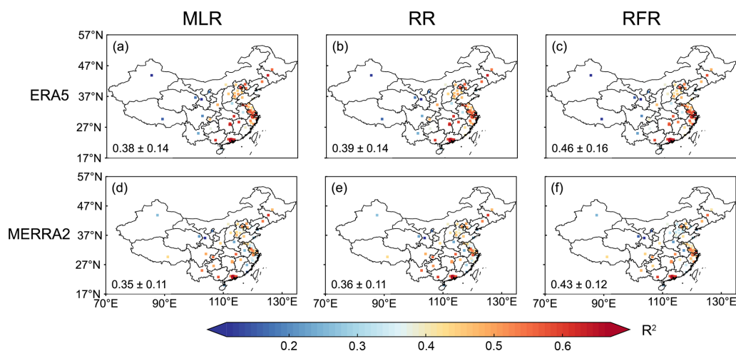
Figure 13. Predictive skills of daily MDA8 ozone in Chinese cities during June to August from 2013 to 2019 by the multiple linear regression (MLR) method, the ridge regression (RR) method, and the random forest regression (RFR) methods, using the meteorological parameters from two re-analysis dataset (ERA5 and MERRA-2). The predictive skills are presented by the coefficient of determination ( R^2 ). Values are the mean \pm standard deviation across 74 cities. See Sect. 2.2 for the descriptions of the three models.
