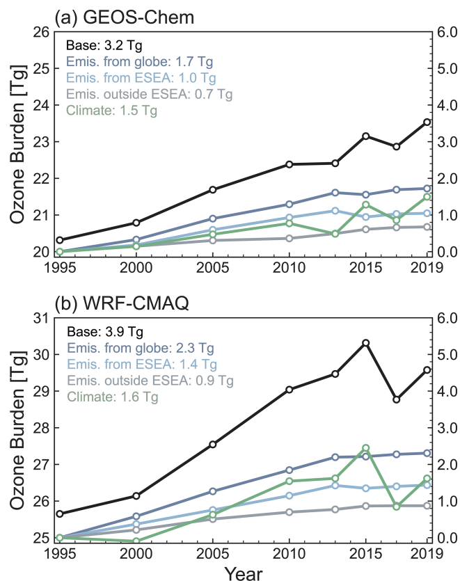
Figure 8. Attribution of summertime tropospheric ozone (represented as tropospheric ozone burden in unit of Tg) in ESEA (including East Asia domain of 80–145° E, 3–53° N and Southeast Asia domain of 92.5–135° E, 10° S–30° N). Results are estimated from the GEOS-Chem and WRF-CMAQ model. Tropospheric ozone burden from the BASE simulation (left y axis) is in absolute values from 1995 to 2019. Changes in tropospheric burden attributed to global anthropogenic emissions (including surface emissions, aircraft emissions, and methane), anthropogenic emissions from ESEA, anthropogenic emissions from other regions, and climate (including biomass burning and stratospheric influences) are values relative to 1995 (right y axis).
