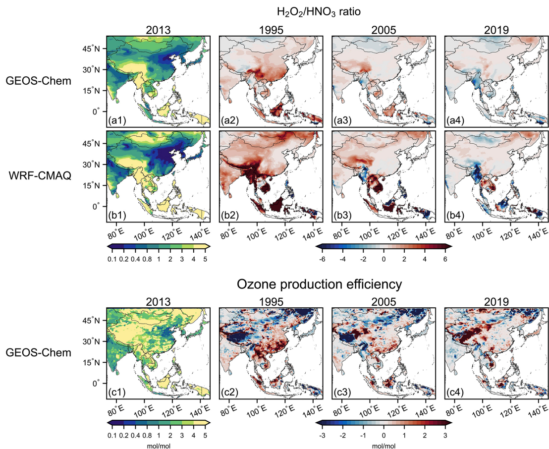
Figure 12. Changes in surface ozone chemical formation regime at the surface in summer 1995–2019. Ozone chemical formation regime is examined using the ratio of \text{H}_2\text{O}_2 to \text{HNO}_3 concentration at the surface. Panels (a1) and (b1) show the spatial distributions in summer 2013 for GEOS-Chem and WRF-CMAQ, respectively, and the rest of the panels show the difference relative to 2013 level.
