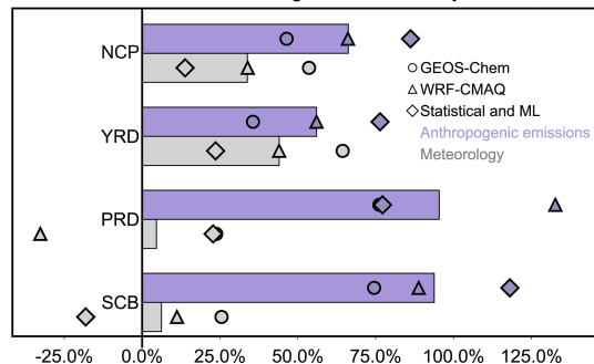
Figure 16. Summary of the meteorology-driven and anthropogenic emission-driven surface MDA8 ozone difference between 2017–2019 and 2013–2015 from the statistical model, machine learning model, and chemical models. Results are summarized from Table 4. The circles and triangles represent result from GEOS-Chem and WRF-CMAQ, respectively. The diamond symbols represent the average of six estimates from the statistical and machine learning model, including three models (MLR, RR, and RFR) with predictions from two meteorological inputs (MERRA-2 and ERA5) in turn. Horizontal bars then represent the mean of the statistical and machine learning model (the ensemble mean from six estimate), GEOS-Chem, and WRF-CMAQ model. See the text for the detailed calculation.
