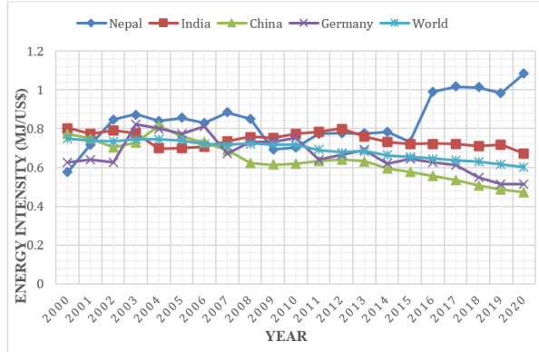
Figure 3: Energy intensity of the commercial and public services GDP value addition of four countries during 2000-2020 (with biomass)
