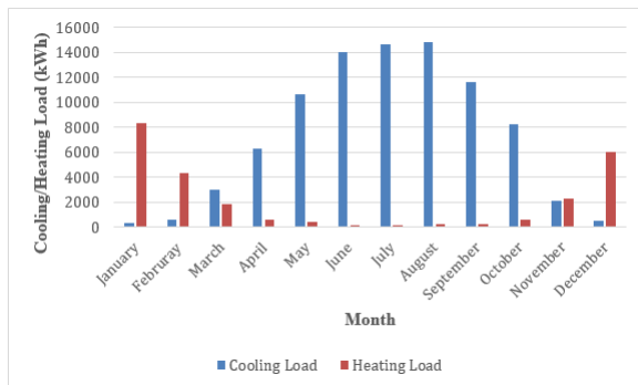
Figure 10: HVAC load profile for efficient case scenario
