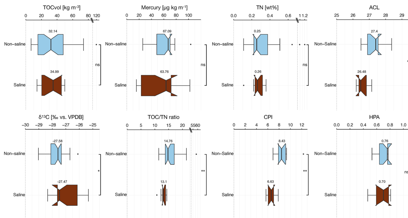
Figure 6. Boxplots of the biogeochemical parameters divided into saline and non-saline sediments: total organic carbon density (TOC vol ) [ \text{kg}_{\text{TOC}} \text{m}^{-3} ], mercury [ \mu\text{g kg}^{-1} ], total nitrogen (TN) in weight per cent [wt %], average chain length (ACL) of n -alkanes, stable carbon isotope ratio [ \delta^{13}\text{C} ] per mil relative to the Vienna Pee Dee Belemnite standard [‰ vs. VPDB], total organic carbon/total nitrogen ratio (TOC/TN ratio), carbon preference index (CPI), and higher plant alcohol index (HPA) of profiles in non-saline (blue) (including upland permafrost, thermokarst lake sediments, and drained lake basin sediments) and saline (red) (including semi-drained lagoon sediments, lagoon sediments, and marine sediments) soil settings. The whiskers display the data range (outliers as black points), and the boxes show the interquartile range (25 %–75 %). The vertical black line marks the median, and the notches represent the 95 % confidence interval. The bars right of the boxes show the statistical significance of differences between the groups (ns: not significant; *: p < 0.05 ; **: p < 0.01 ; ***: p < 0.001 ).
