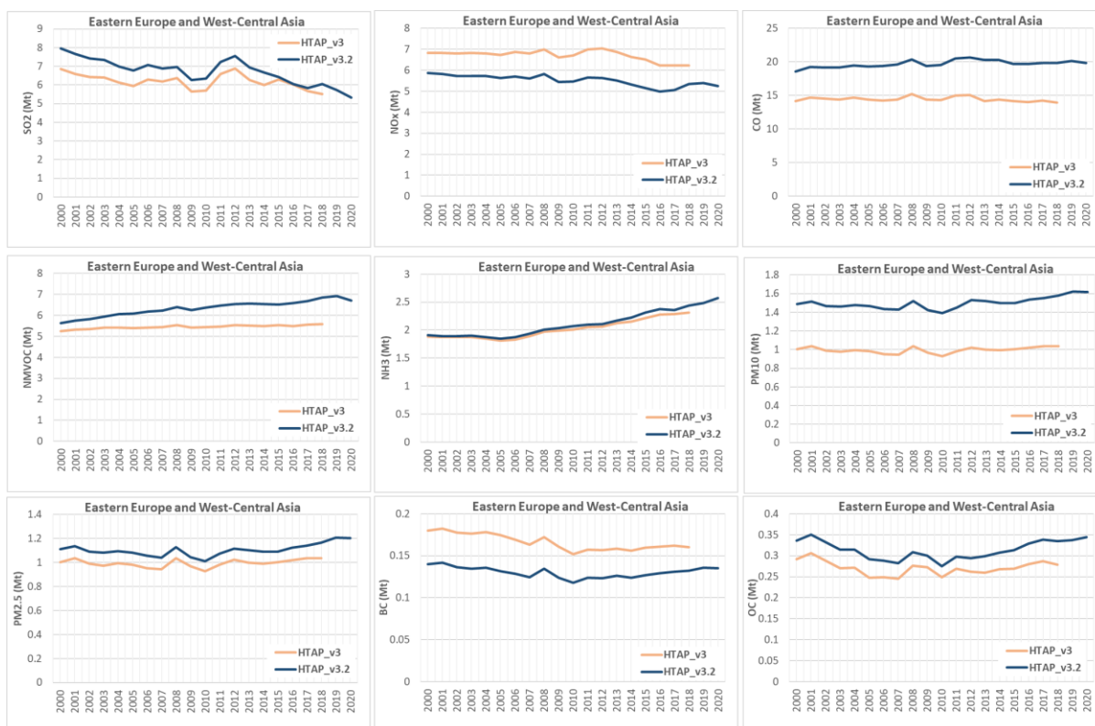
Figure S14 – Comparison of HTAP_v3 and HTAP_v3.2 emissions for Eastern Europe and West-Central Asia.
