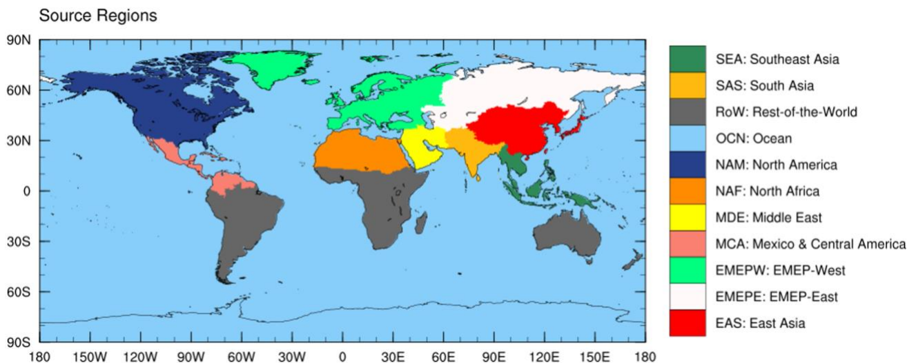
Figure 1 The HTAP3 source regions.
